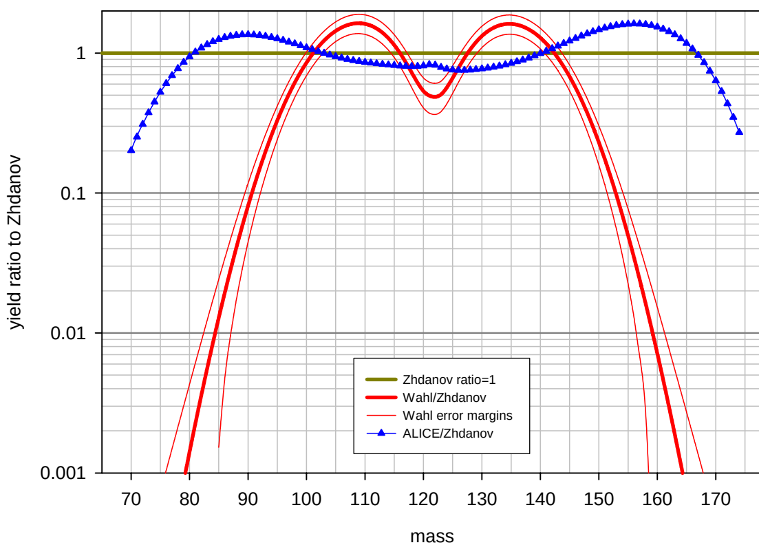
Benchmark B: ^{244}\text{Cm} at 28 MeV, pre-neutron emission yield ratio to Zhdanov's data
